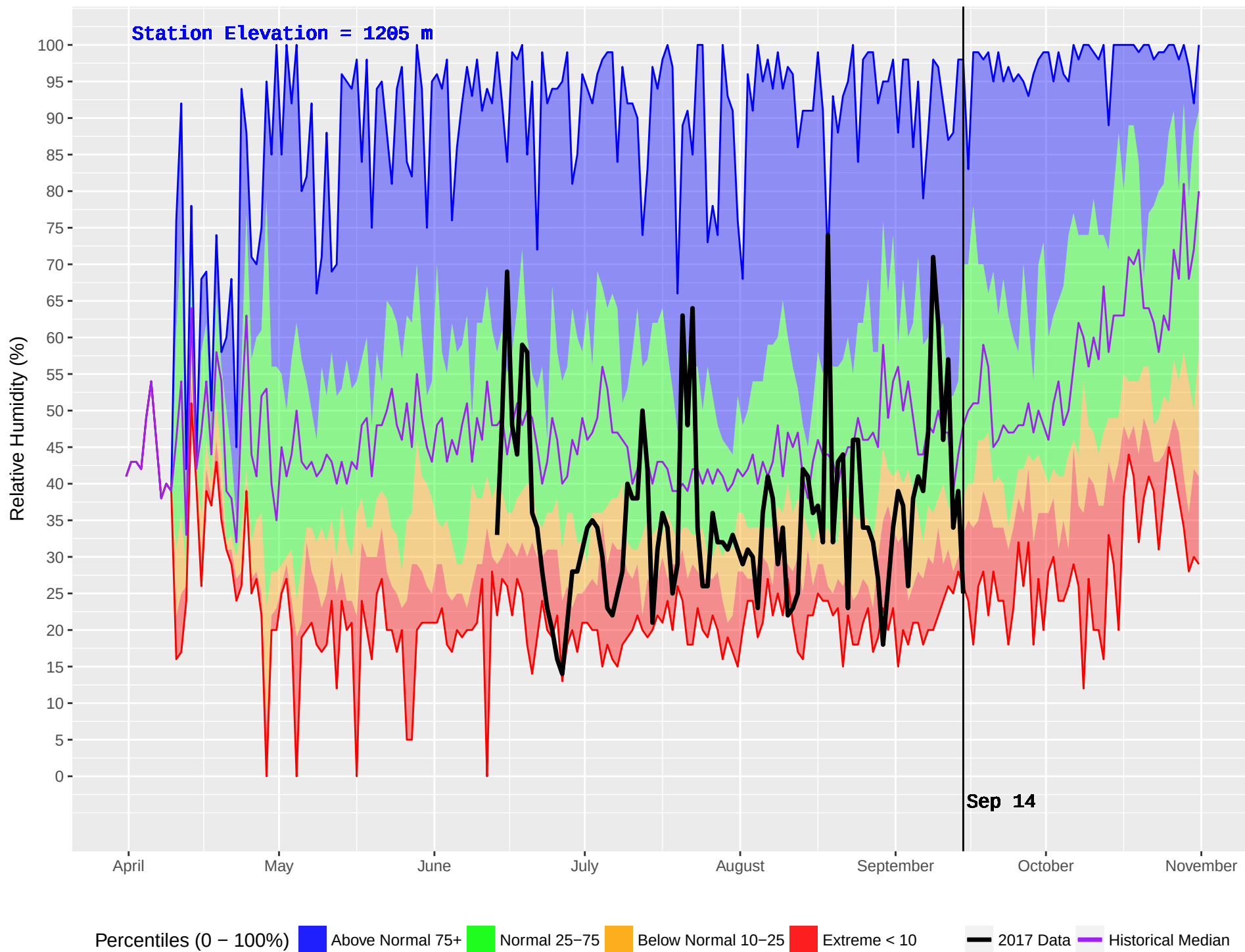
GWYNETH LAKE (309) : Historical (1986–2016) and Current (2017) Noon Relative Humidity
